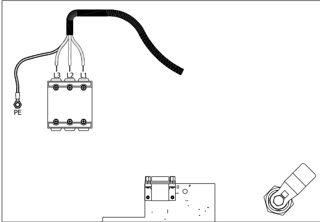
MG 18 input cord connection(maximum screwing torque is 0.8Nm)
