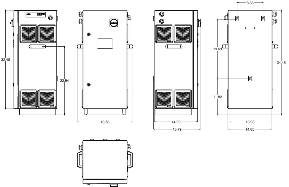
Mechanical dimension and drilling details MG18
