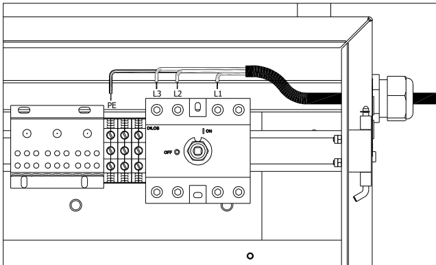
MG 27/36 input cord connection(maximum screwing torque is 10Nm)
