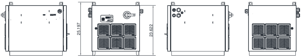
Mechanical dimension MG27
