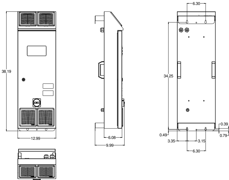
Mechanical dimension and drilling details MG 9
