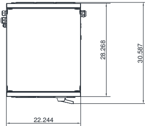
Mechanical dimension MG36
