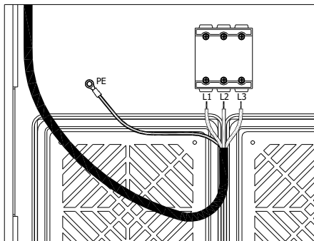
MG 9 input cord connection(maximum screwing torque is 0.8Nm)
